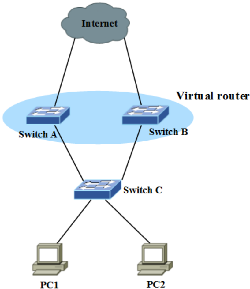
Figure 1. VRRP Networking Diagram
