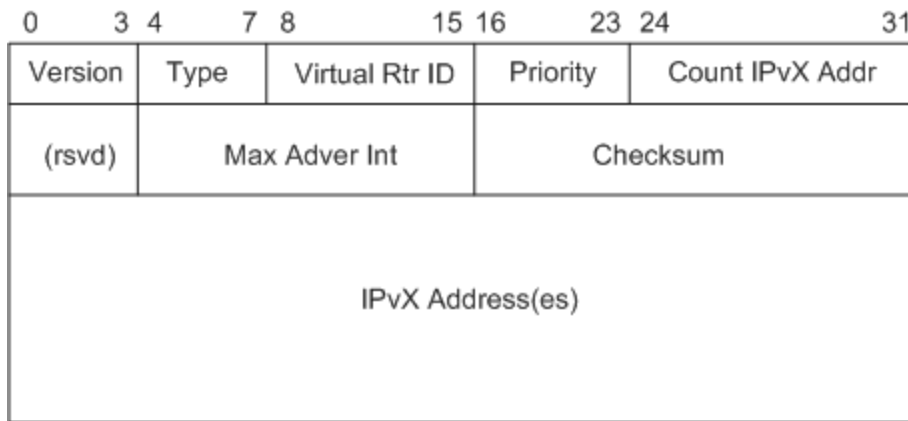
Figure 3. VRRPv3 Packet
