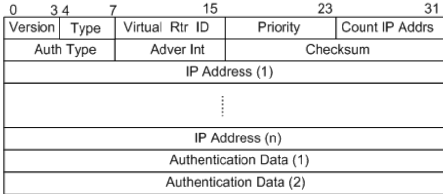
Figure 2. VRRPv2 Packet
